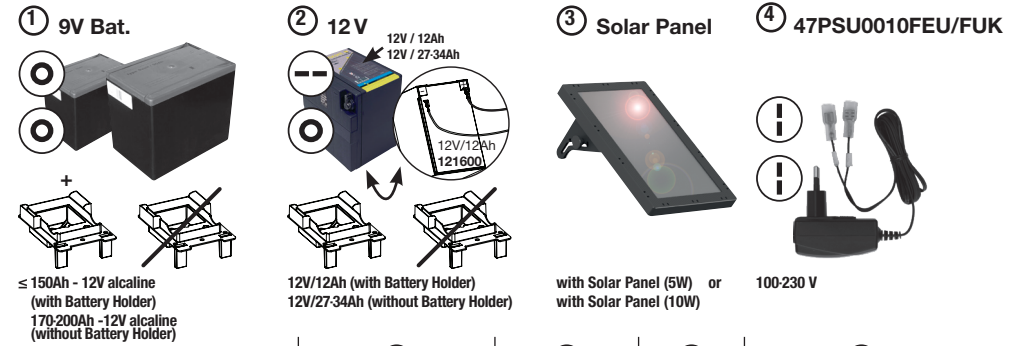
Fig. 3 OPTIONAL MINIMUM POWER SUPPLY:
